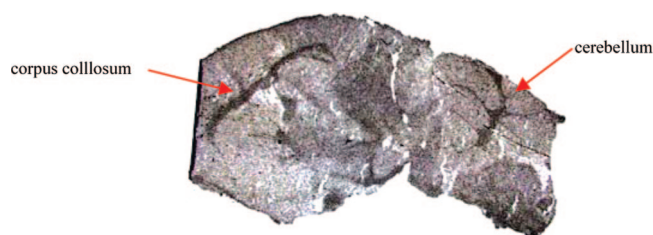
Figure 7. Film autoradiography shows [ ^{125} I] 9 binding to myelinated corpus callosum and cerebellum in mouse brain sections (sagittal). Arrows show myelinated corpus callosum (A) and cerebellum (B) labeled by [ ^{125} I] 9 .
